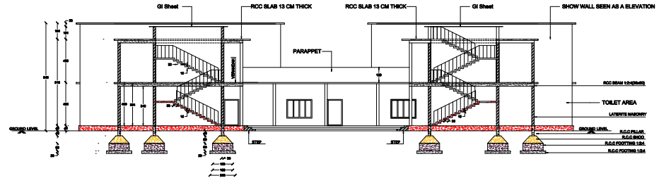
SECTION XX
